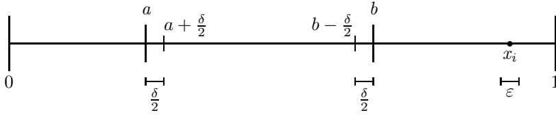
Figure 1. The gappy model, showing parameters a and b stated to precision \frac{\delta}{2} , and one data point x_i stated to accuracy \varepsilon .
