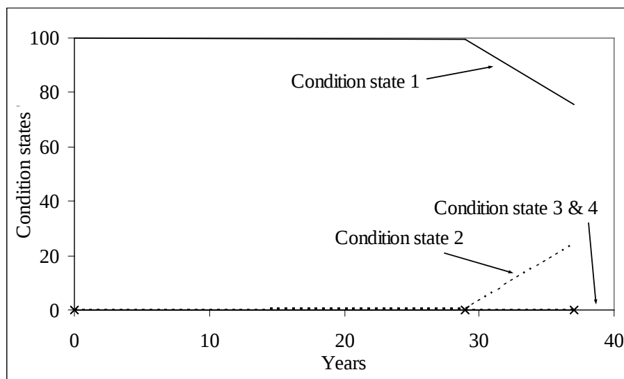
Fig. 3. Deterioration model for the bridge element 8P
